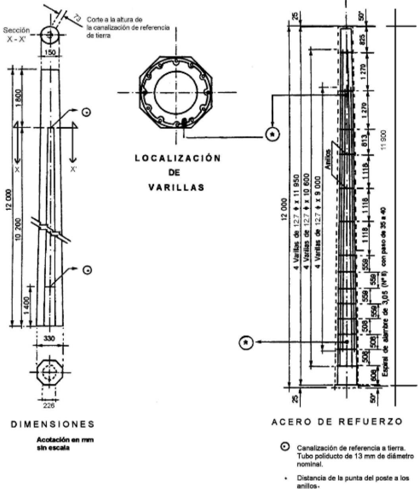
FIGURA 8 – Poste PCR-12-750
