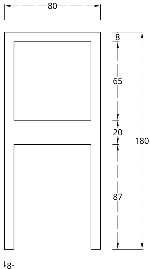
VISTA FRONTAL
