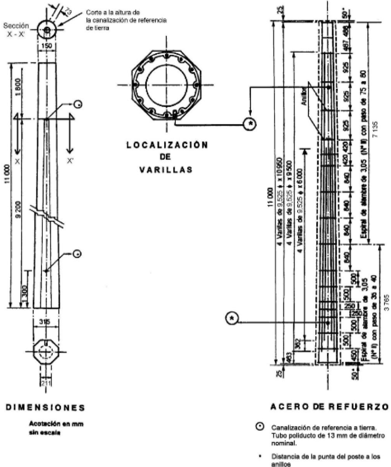
FIGURA 6 – Poste PCR-11-500
